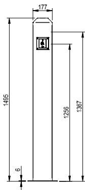
WRMPExSNxx One Wall Reader
