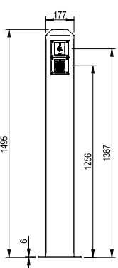
WRMPExSKxx One Wall Reader and Key pad
