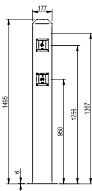
WRMPExDNxx Two Wall Readers DDA compliant
