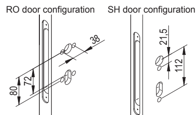
DL = For deadlatches
