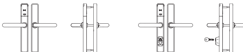
Clutch mechanism
