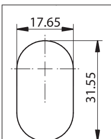
K cam
