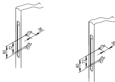
SH= Short plate configuration
