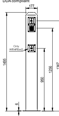
WRMPExDKxx Two Wall Readers and one Key pad. DDA compliant
