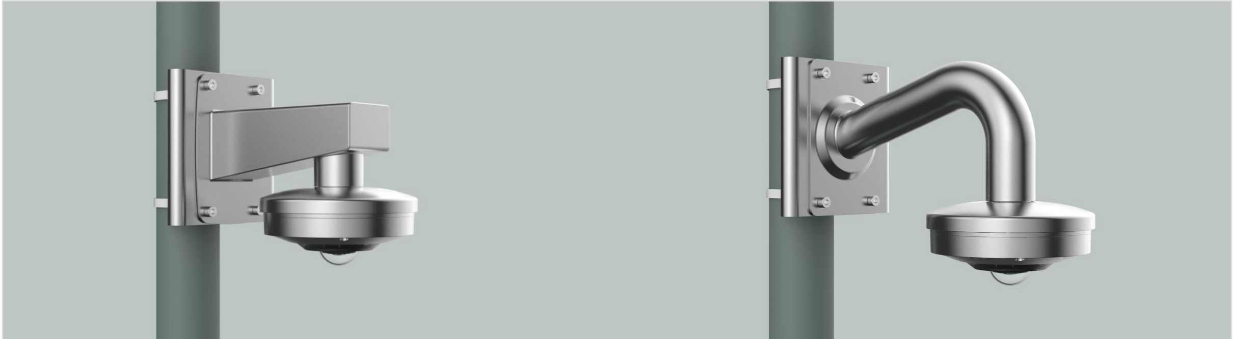
Pole Mount
